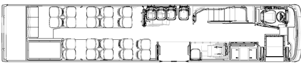
Lower deck with 23 fixed seats, 5 tip-up seats + 2 wheelchair positions
